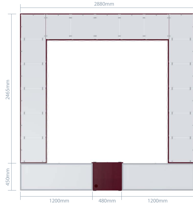
TOP VIEW
